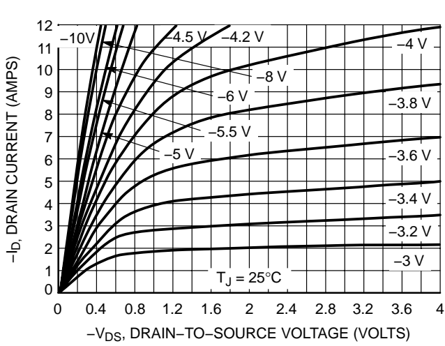
Figure 4. On-Region Characteristics
